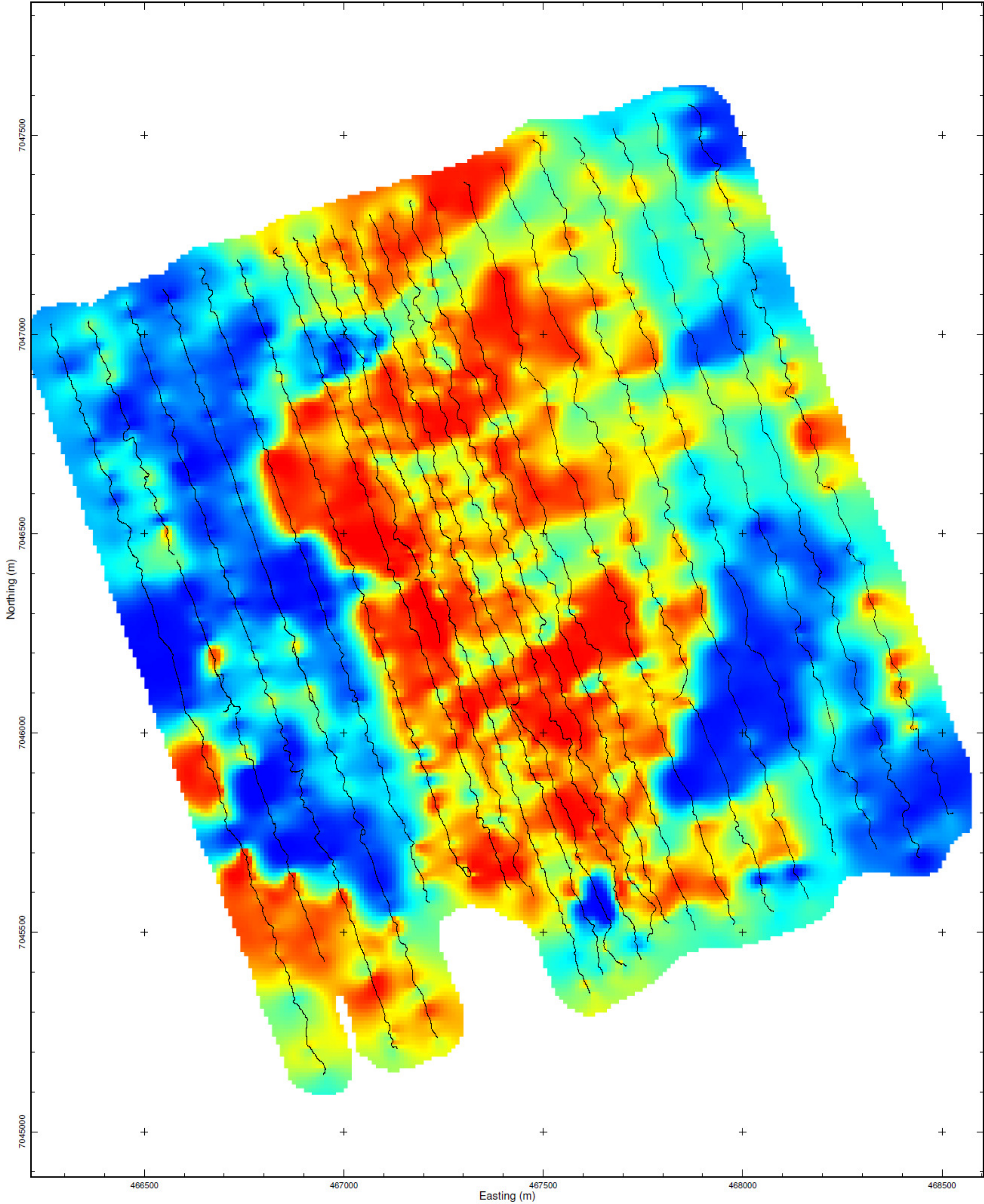
EM38 Conductivity Data
